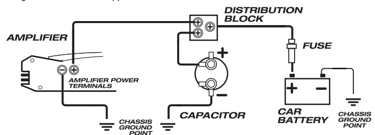
SUGGESTED WIRING
