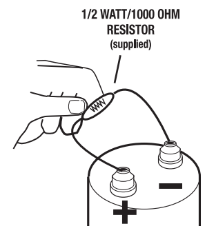
Discharging the capacitor
