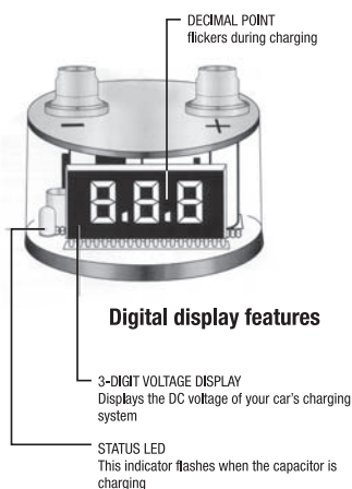
Charging the capacitor
