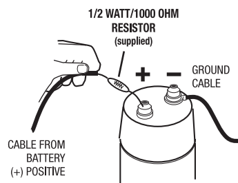
Charging the capacitor
